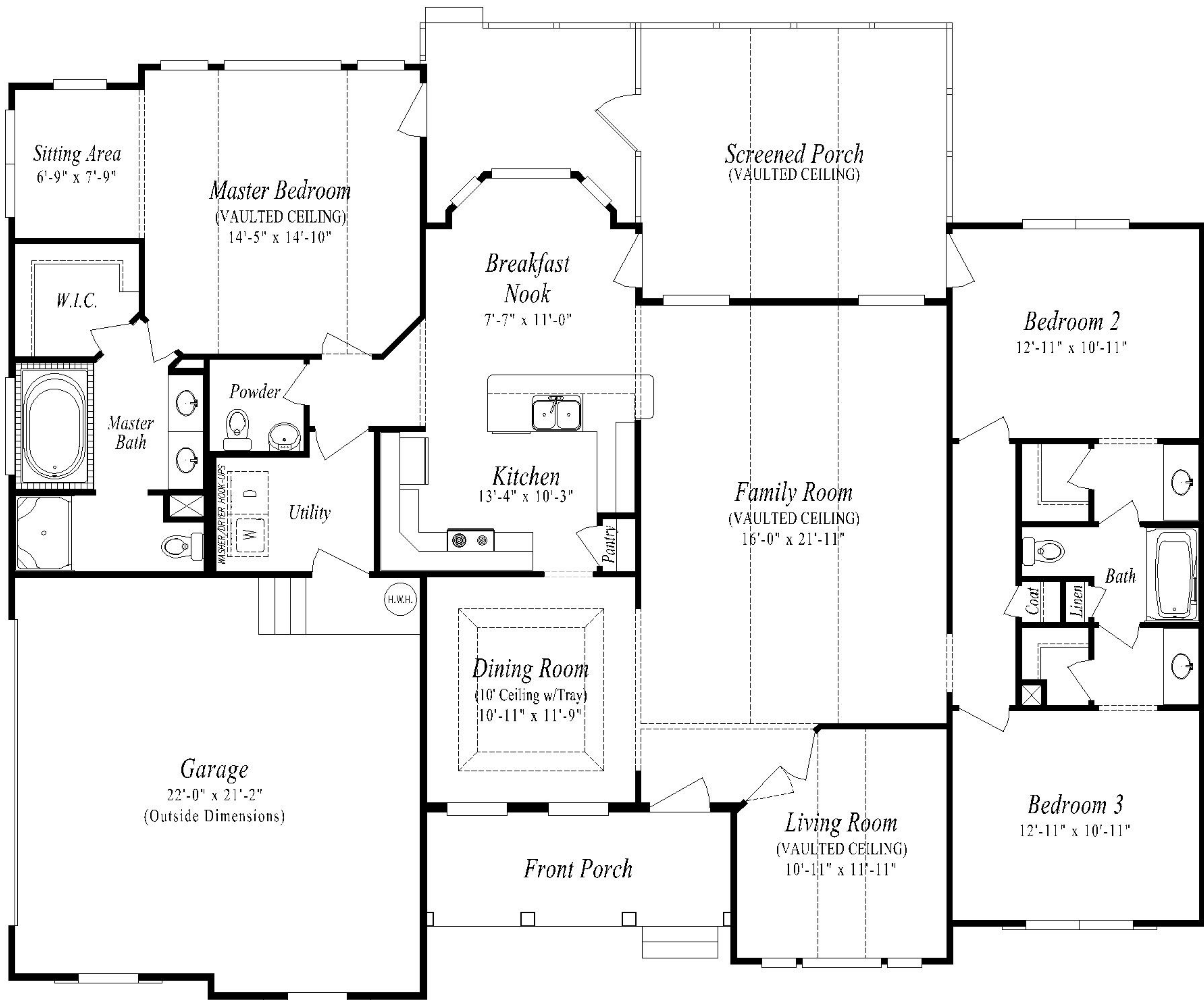
Floor Plan
