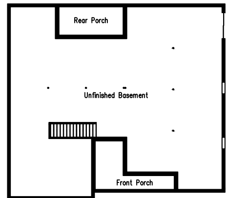
Optional Basement/ Foundation Plan Standard Foundation is Crawl Space
