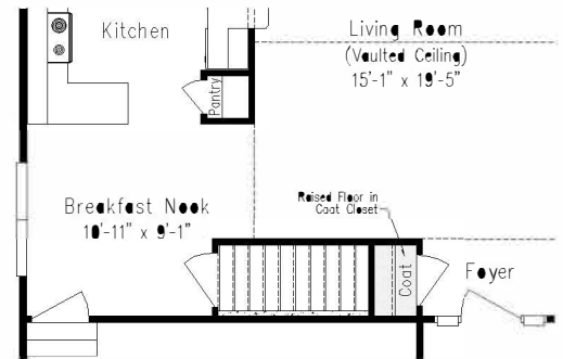
Partial Floor Plan with Optional Basement Stairs
