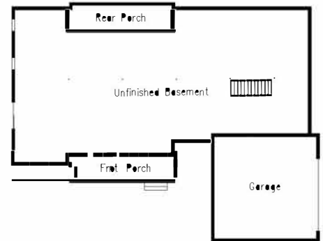
Optional Basement/ Foundation Plan Standard Foundation is Crawl Space
