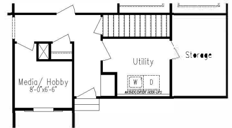
Partial Floor Plan with Basement Stairs
