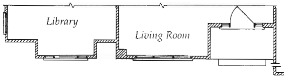
Partial First Floor Plan w/Elev.3
