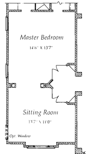
Partial Plan w/Opt. Sitting Room
