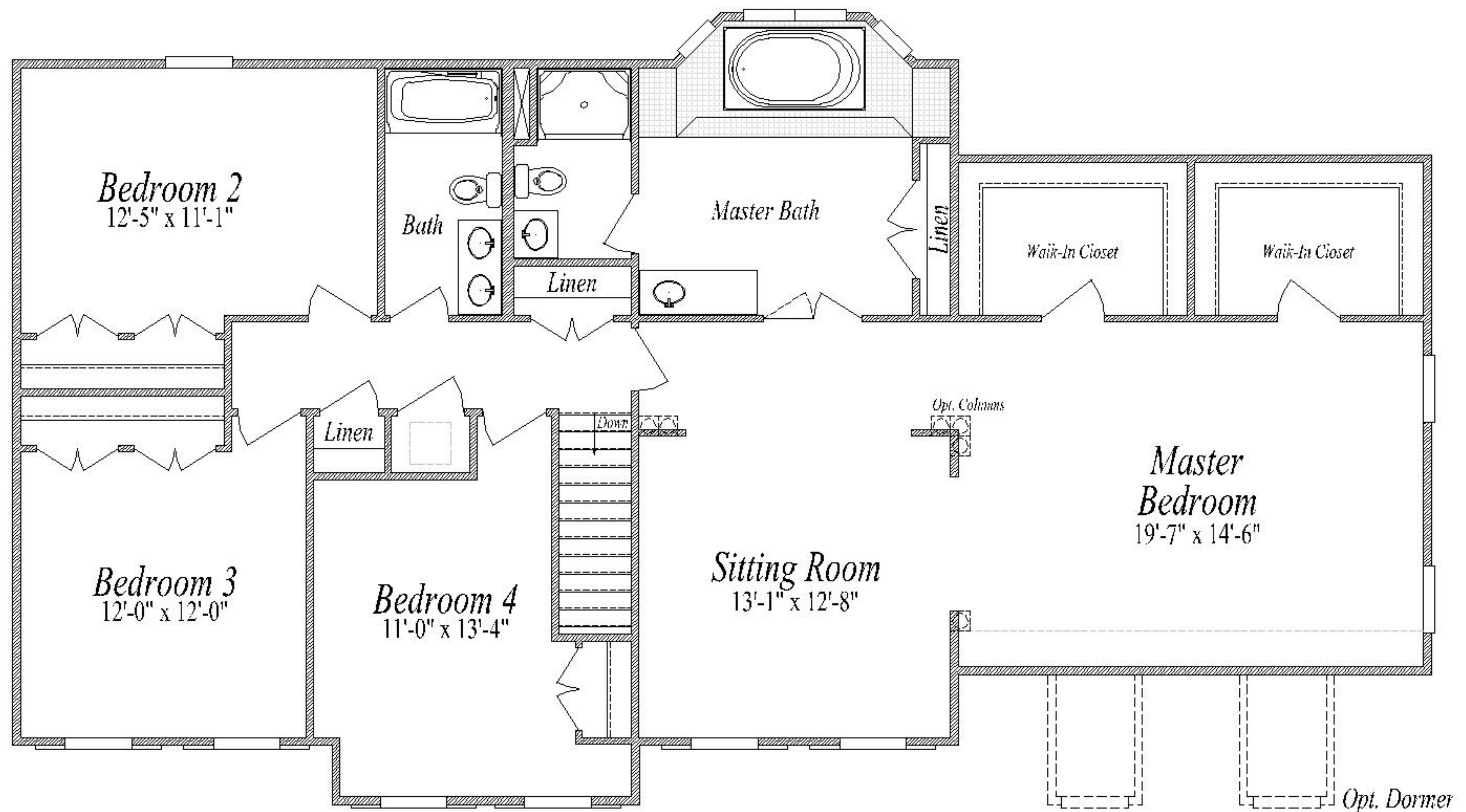
Opt. Master Suite Floor Plan
