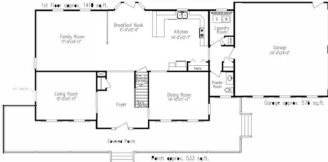
1st Floor approx. 1410 sq.ft.
