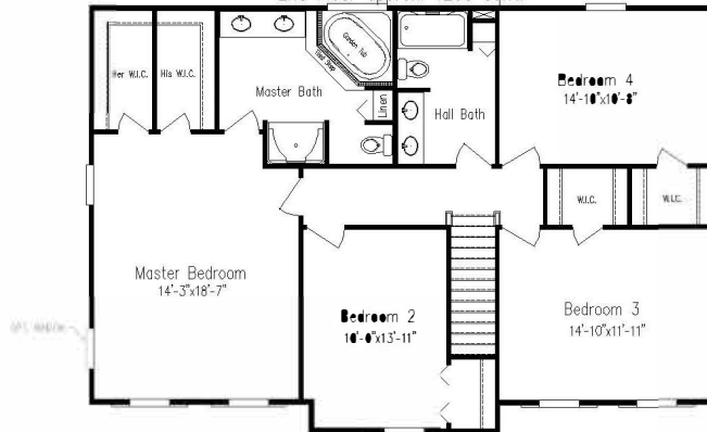
2nd Floor approx. 1258 sq.ft.
